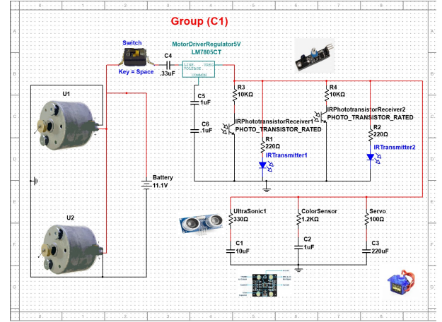
Fig. 10. Multisim simulation
